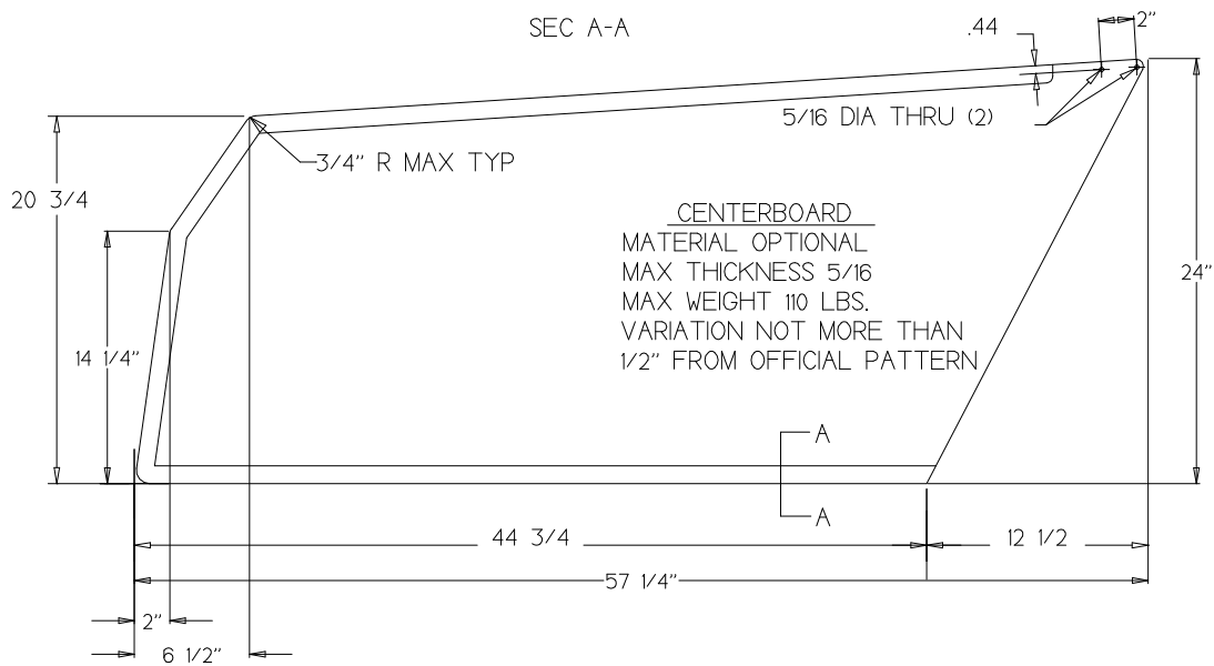
CENTERBOARD
